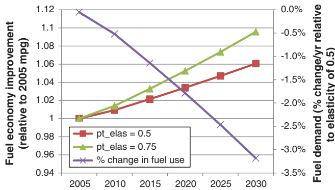
Fig. 6. Simulated improvement in the vehicle fleet fuel economy (both new and used vehicles) and total fuel use using alternative elasticities of substitution between fuel and powertrain capital ( \sigma_{F,K_{PT}} (pt_elas) = 0.5, 0.75) in the MIT EPPA model in a reference (no policy) scenario.
