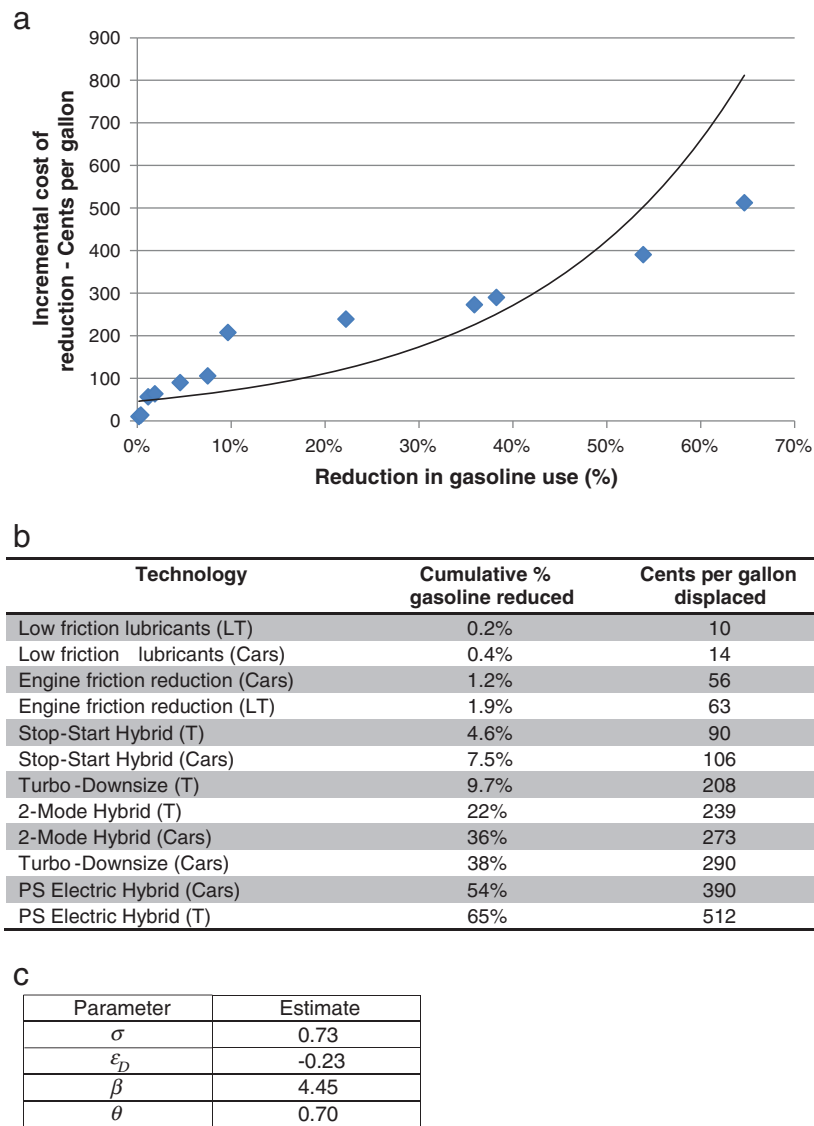
Fig. 5. Technology-response curves for passenger vehicles in 2011, with a) incremental cost of reducing fuel use through application of technology graphed against cumulative fuel use reduction, b) the table of cost-effectiveness values from EPA (2010) used to parameterize the curve for light-duty vehicles (cars and light-duty trucks), and c) estimated values of the substitution elasticity and related variables for each curve.
